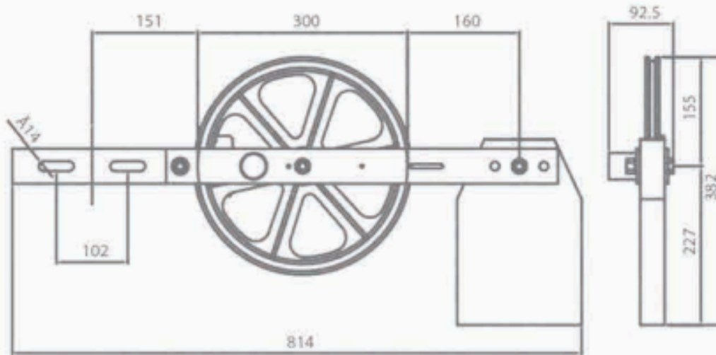
Rope Tensioner without guard
