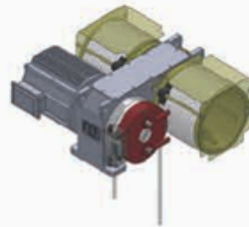
A-type 268H: Upward mounted horizontal downward rope outlet
