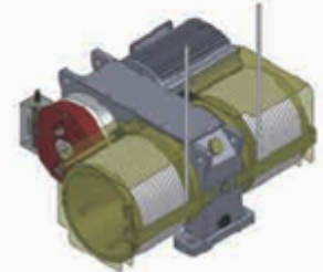
C-type 268H: Bottom mounted horizontal upward rope outlet
