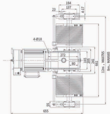
PRO1128-8-12m mounting dimension
